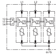
Basic circuit diagram DG MU 3PY 480 3W+G R
