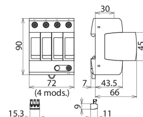
Dimension drawing DG MU 3PY 600 4W+G R
