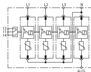
Basic circuit diagram DG MU 3PY 600 4W+G R
