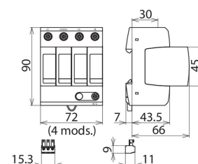
Dimension drawing DG MU 3PH 480 4W+G R
