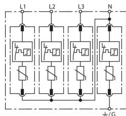
Basic circuit diagram DG MU 3PY 480 4W+G
