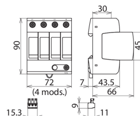
Dimension drawing DG MU 3PY 208 4W+G R
