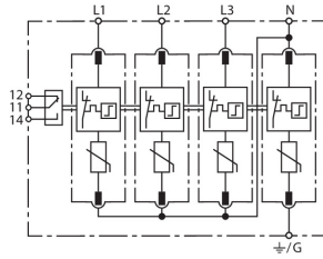
Basic circuit diagram DG MU 3PY 480 4W+G R
