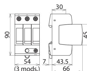
Dimension drawing DG MU 3PD 240 3W+G
