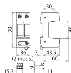
Dimension drawing DG MU SP 240 3W+G R
