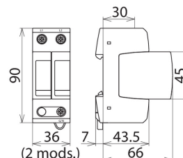
Dimension drawing DG MU CGD 480 3W+G
