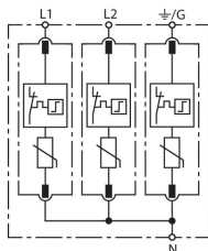
Basic circuit diagram DG MU SPN 240 3W+G
