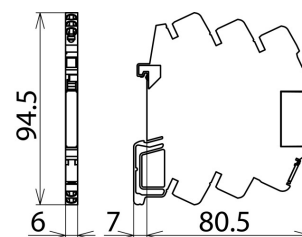
Dimension drawing DCO SD2 ME 12
