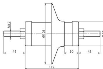
Dimension drawing DMI 6 10 1 N
