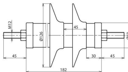
Dimension drawing DMI 18 10 1 N
