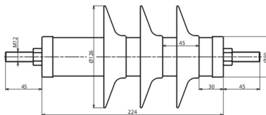
Dimension drawing DMI 24 10 1 N
