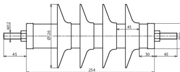
Dimension drawing DMI 30 10 1 N
