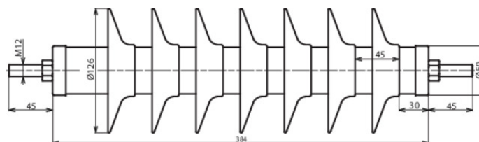
Dimension drawing DMI 39 10 1 N
