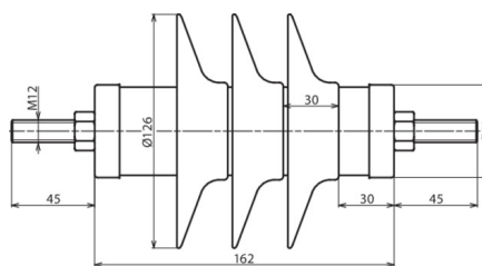
Dimension drawing DMI 15 10 1 H
