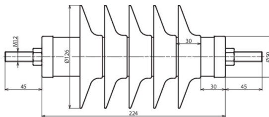
Dimension drawing DMI 24 10 1 H
