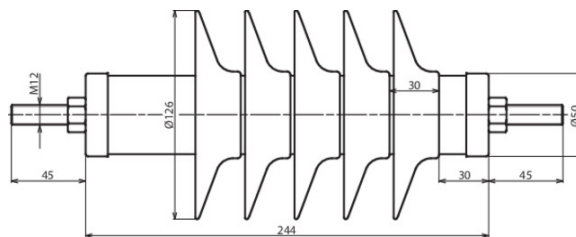
Dimension drawing DMI 27 10 1 H
