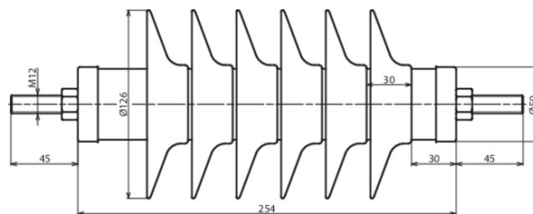
Dimension drawing DMI 30 10 1 H
