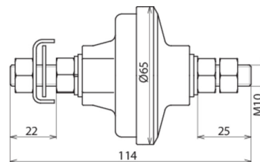
Dimension drawing DIC 10
