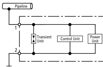
Basic circuit diagram VCSD 40 IP65
