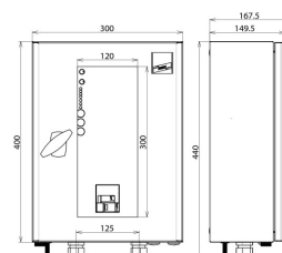
Dimension drawing VCSD 40 IP65
