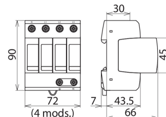
Dimension drawing DG M TNS 275 NL FM
