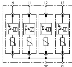
Basic circuit diagram DG M TNS 275 NL FM
