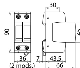
Dimension drawing DG M TT 2P 275 NL
