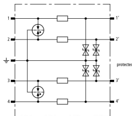
Basic circuit diagram BSP M4 BE 48
