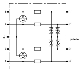
Basic circuit diagram BSP M4 BE 60
