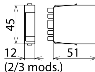
Dimension drawing BSP M4 BE 60
