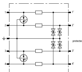
Basic circuit diagram BSP M4 BE 180
