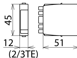
Dimension drawing BSP M4 BE 180
