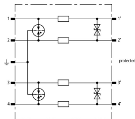
Basic circuit diagram BSP M4 BD 5
