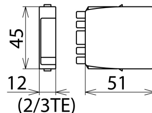
Dimension drawing BSP M4 BD 5
