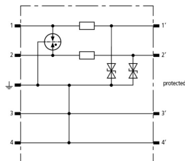
Basic circuit diagram BSP M2 BE 24
