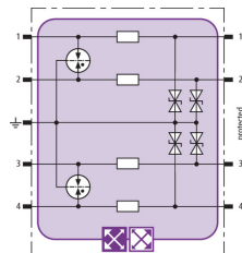
Basic circuit diagram BXT ML4 BE 60
