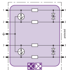
Basic circuit diagram BXT ML4 BD 5
