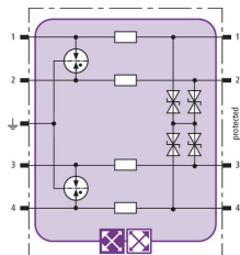
Basic circuit diagram BXT ML4 BC 5
