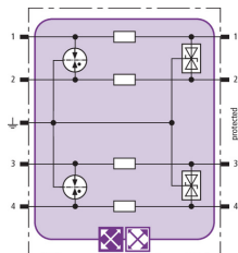
Basic circuit diagram BXT ML4 BE HF 5
