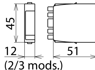
Dimension drawing BXT ML2 BE S 48
