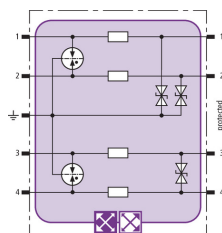
Basic circuit diagram BXT ML4 BE BD 24
