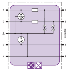
Basic circuit diagram BXT ML2 BE S 36
