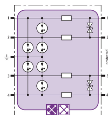
Basic circuit diagram BXT ML4 BD EX 24
