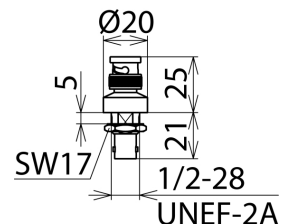
Dimension drawing DGA G BNC
