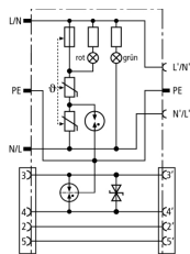
Basic circuit diagram DPRO 230 NT
