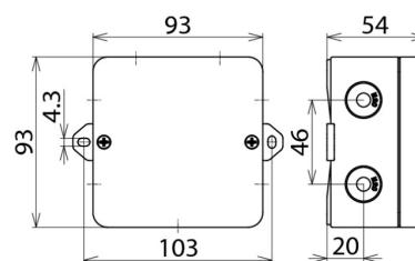
Dimension drawing DBX TC 180
