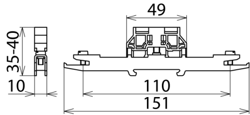
Dimension drawing SH2 18X3 ST
