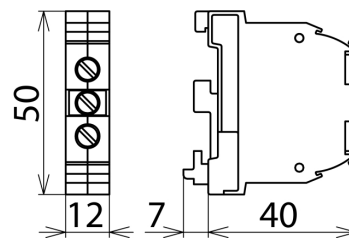
Dimension drawing SLK 16
