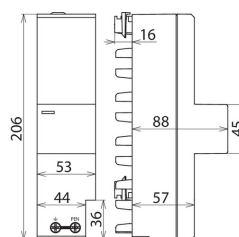
Dimension drawing DSH ZP B TNC 255
