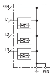
Basic circuit diagram DSH ZP B TNC 255
