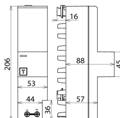
Dimension drawing DV ZP TT 255
