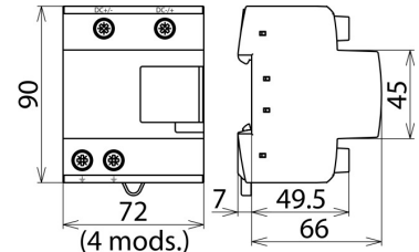
Dimension drawing DCB YPV SCI 1000
