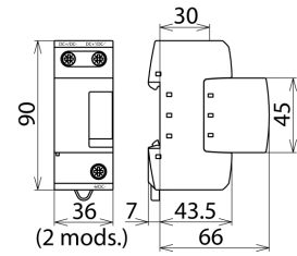
Dimension drawing DSE M 1 220
