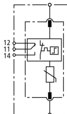
Basic circuit diagram DG S WE 600 FM
