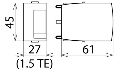
Dimension drawing DG MOD E H 1000 VA
