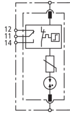
Basic circuit diagram DG MOD E H 1000 VA
