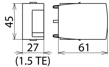
Dimension drawing DG MOD E CI 440
