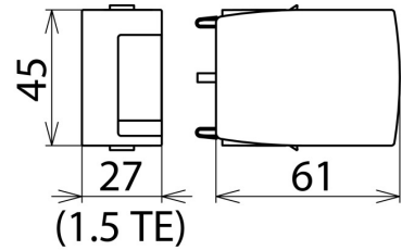
Dimension drawing DG MOD E CI WE 440
